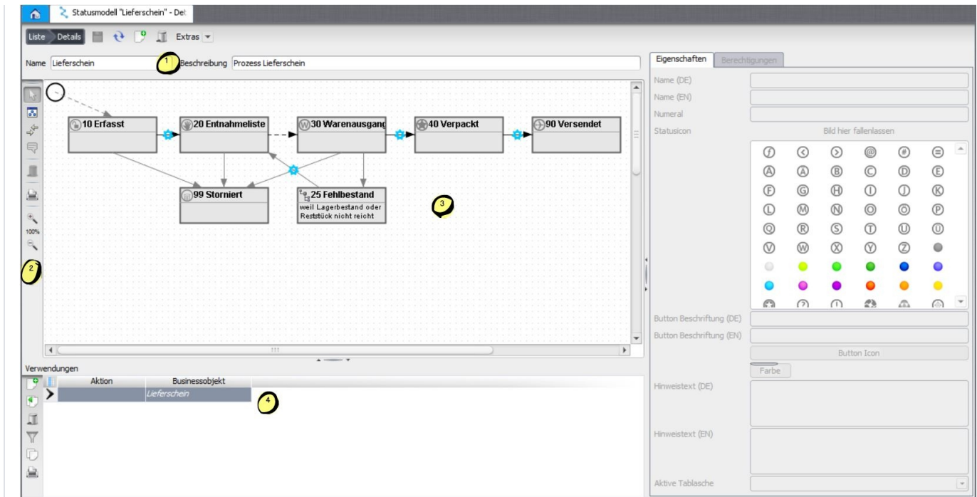
Status model editor: states and transitions.
